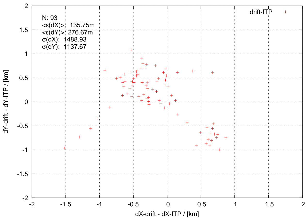
itp61 20130401 to 20130630
