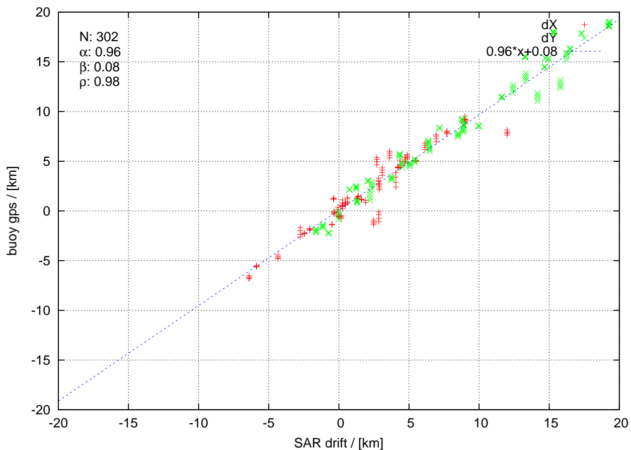
itp60 20130401 to 20130630
