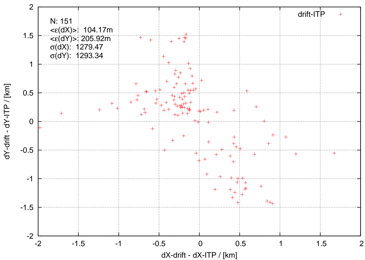
itp60 20130401 to 20130630
