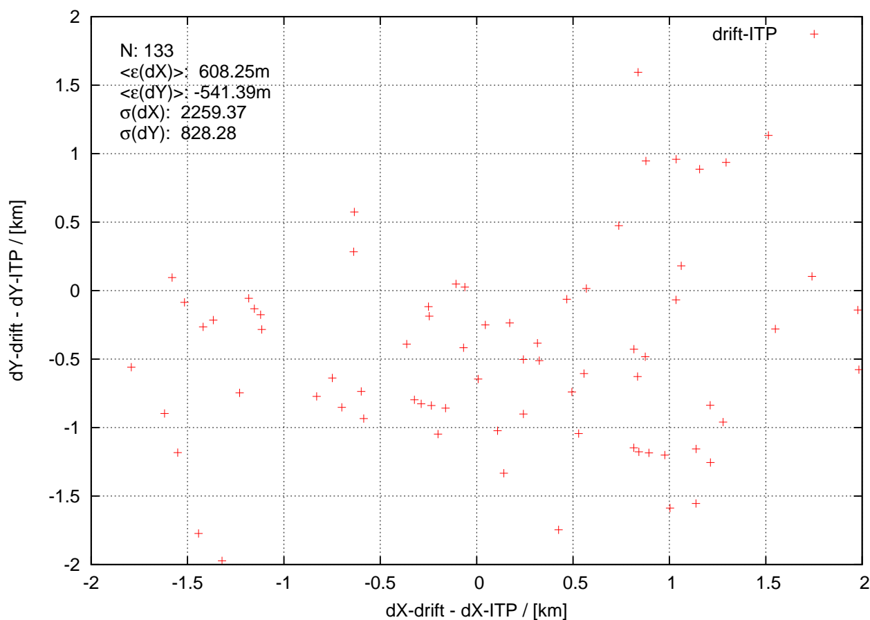
itp49 20130401 to 20130630
