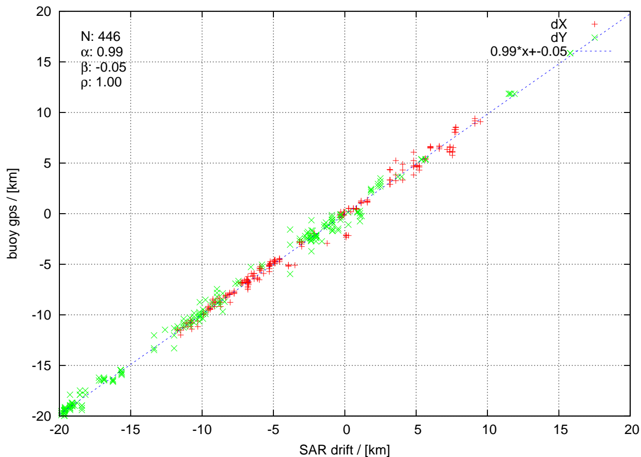
itp74 20141001 to 20141205
