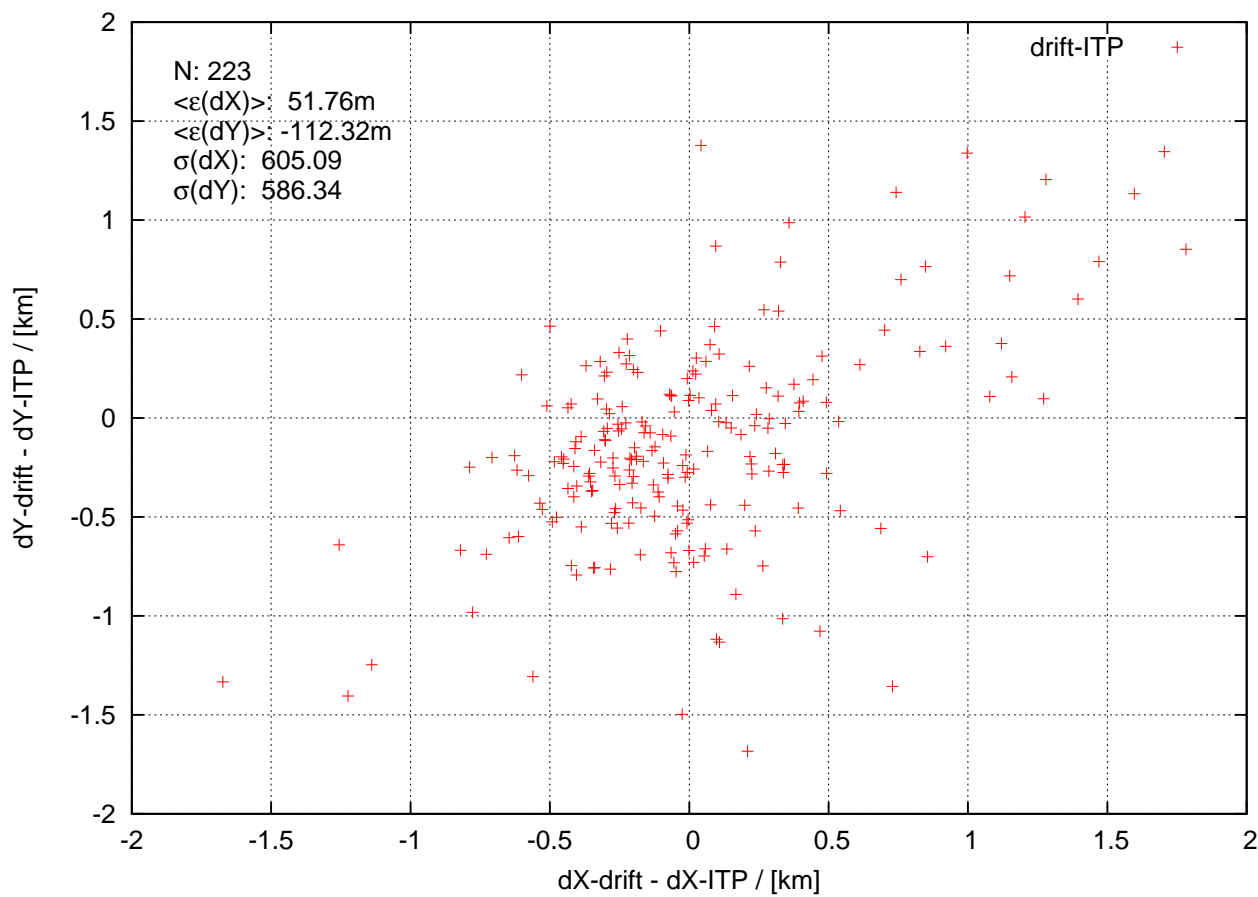
itp74 20141001 to 20141205
