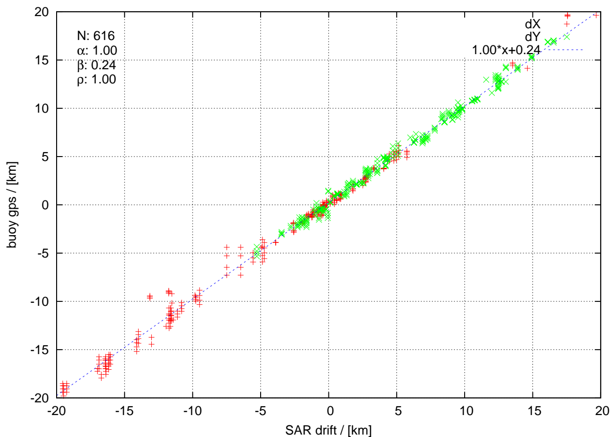
itp76 20141001 to 20141205
