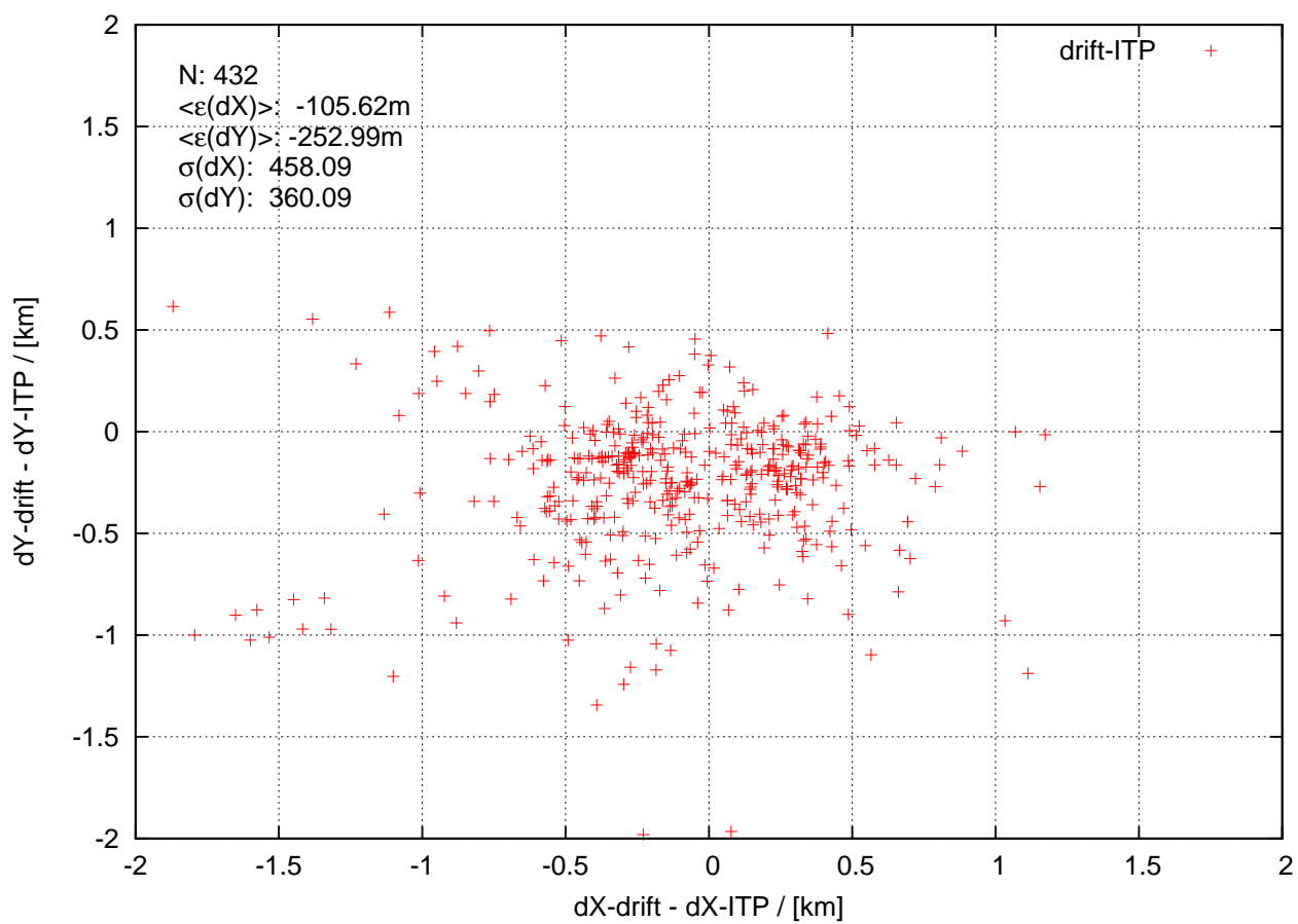
itp75 20141001 to 20141205
