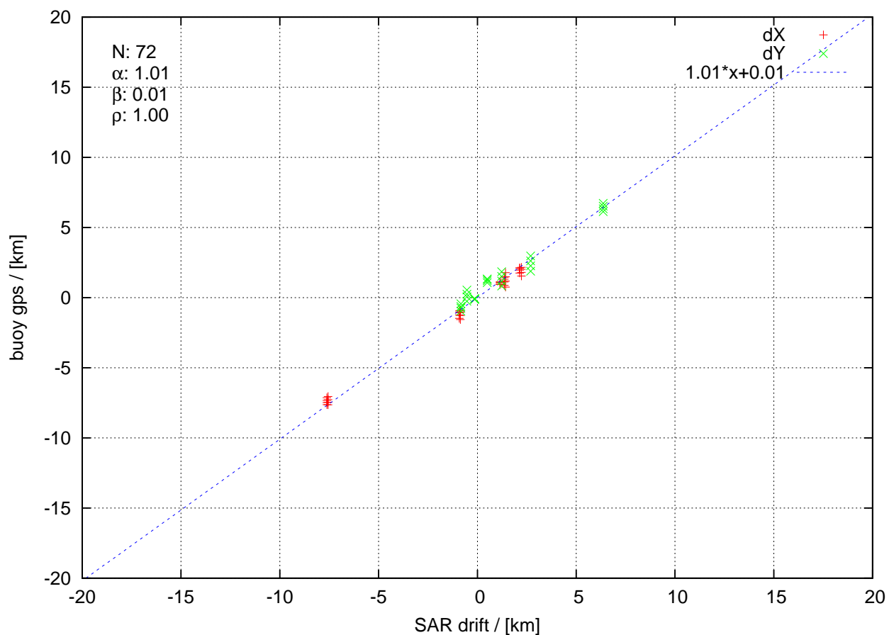
itp59 20141001 to 20141205
