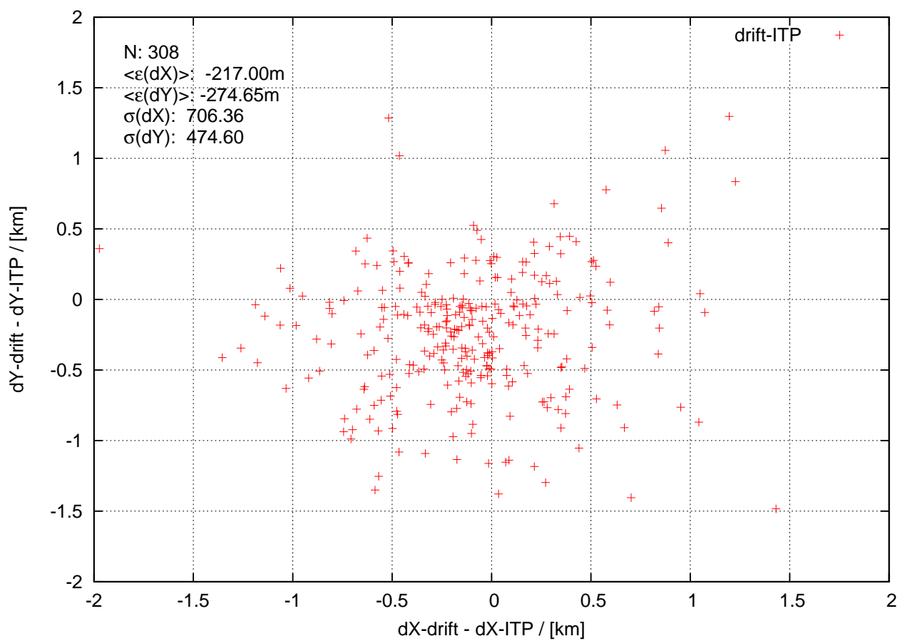
itp76 20141001 to 20141205
