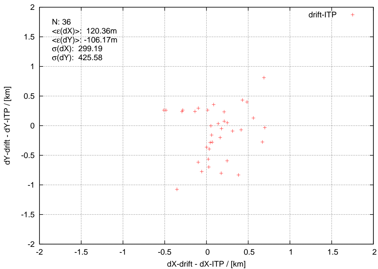
itp59 20141001 to 20141205
