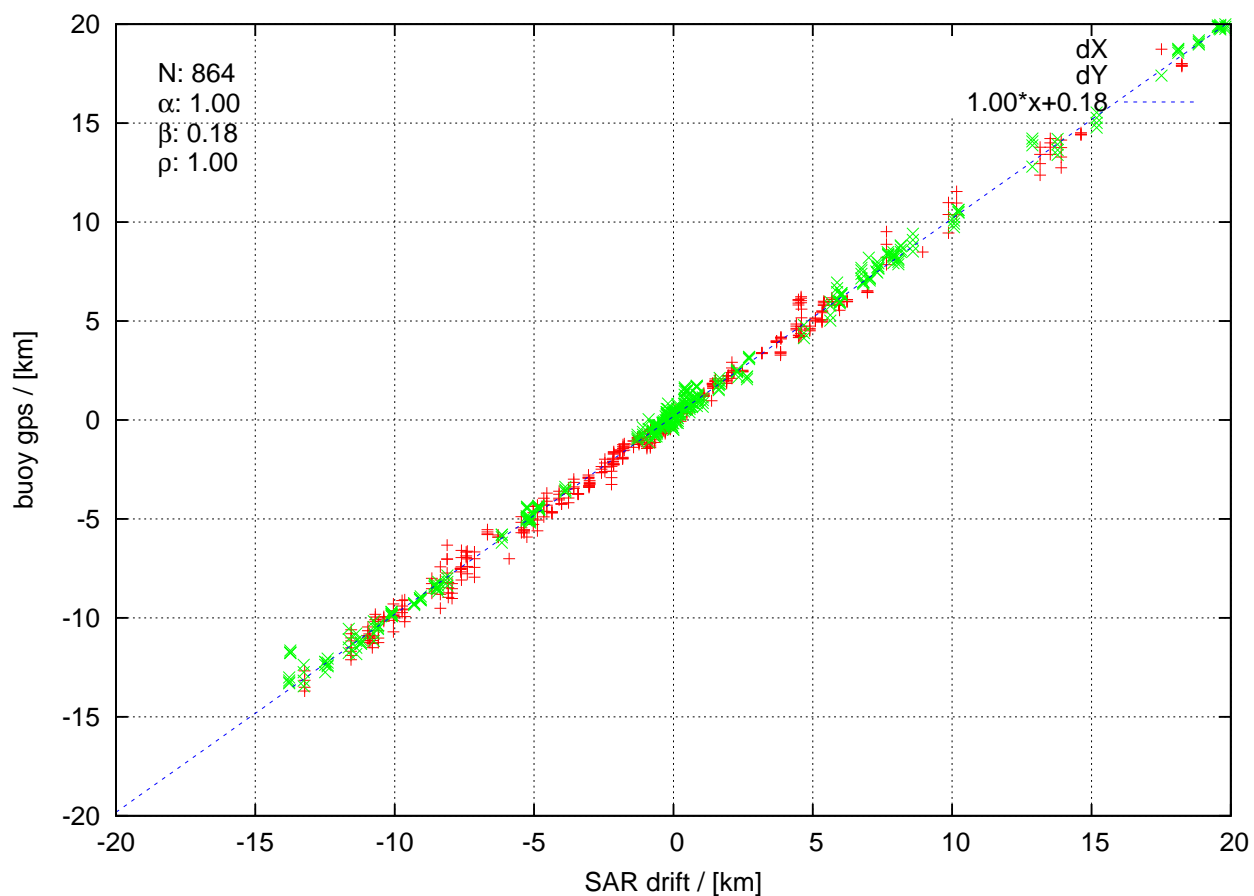
itp75 20141001 to 20141205
