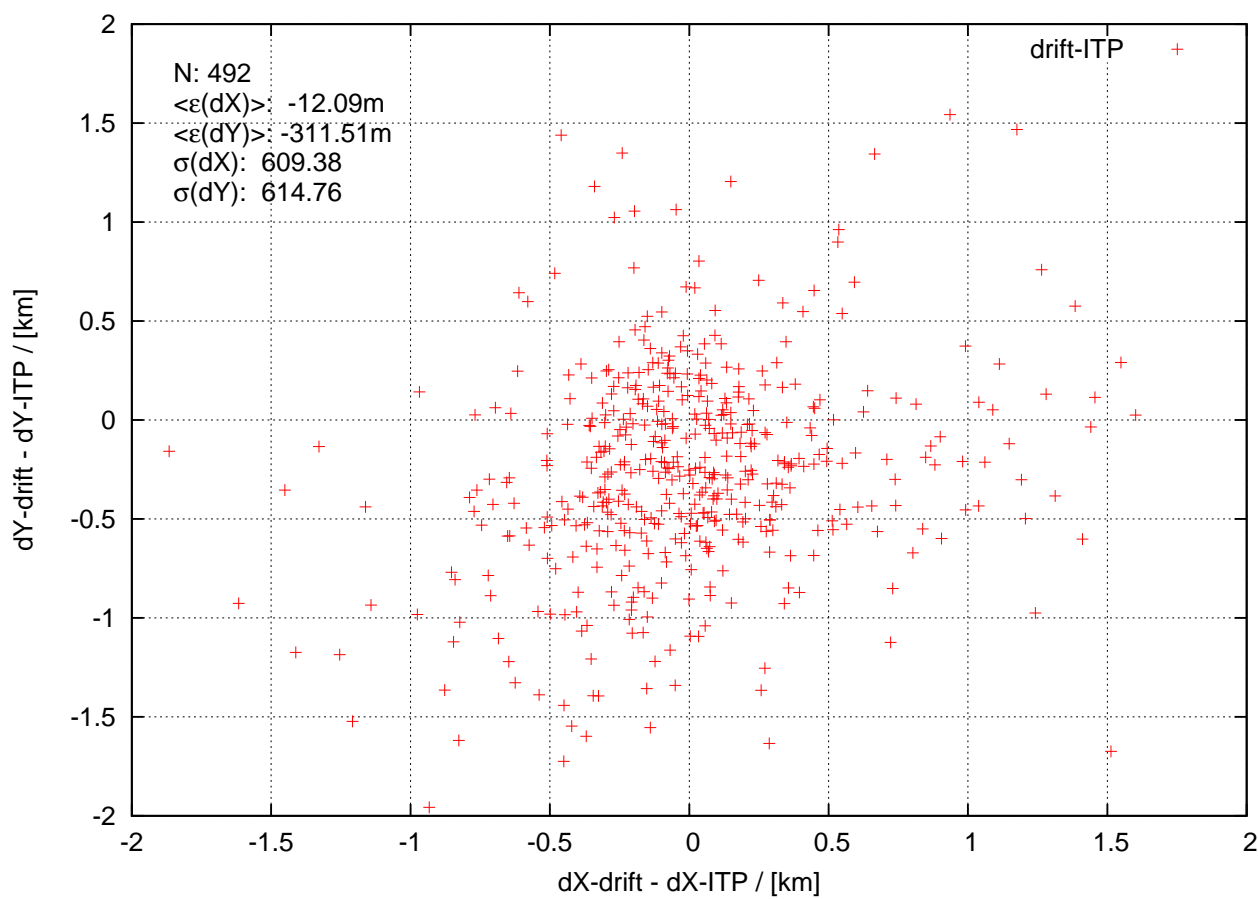
itp72 20141001 to 20141205
