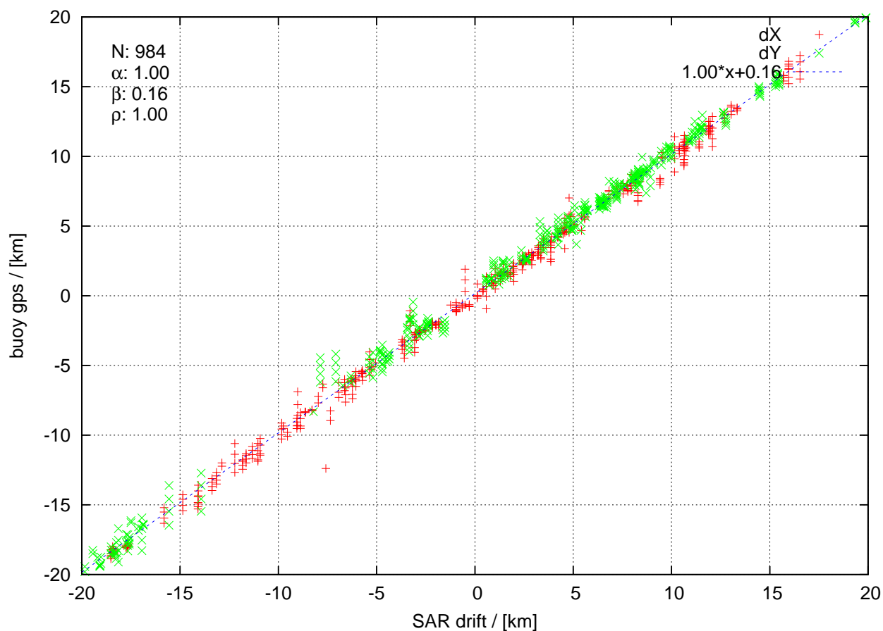
itp72 20141001 to 20141205
