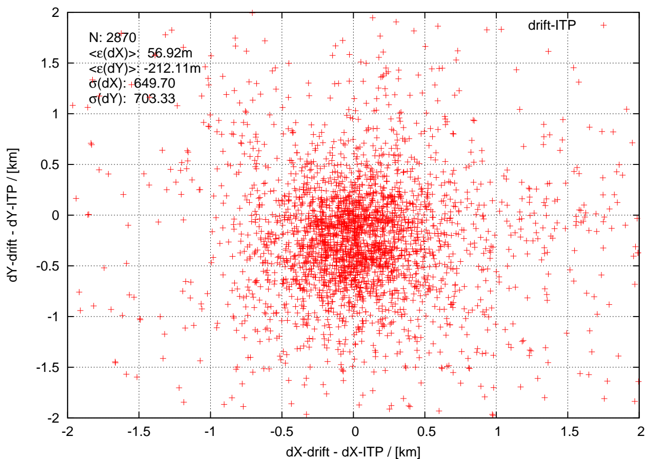
itp91 20160703 to 20160930
