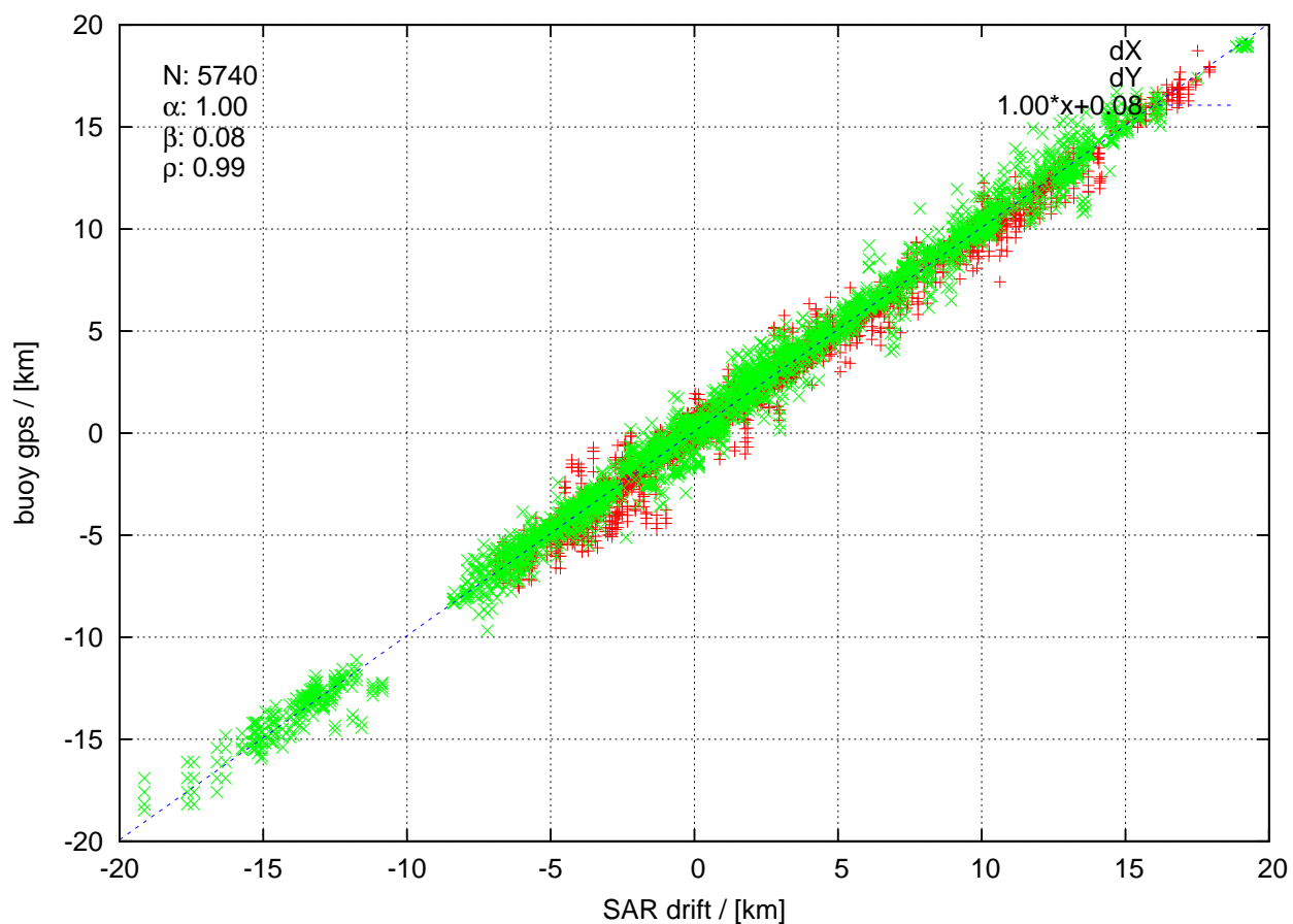
itp91 20160703 to 20160930
