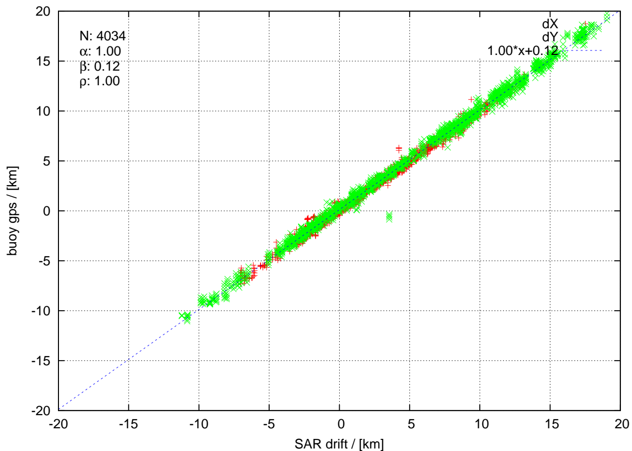
itp93 20160703 to 20160930
