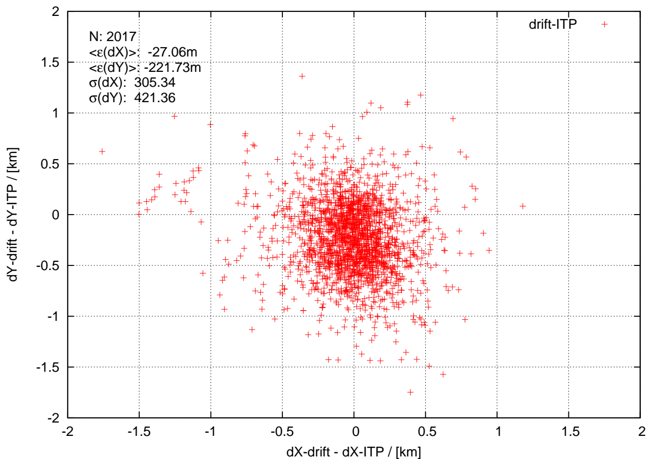
itp93 20160703 to 20160930
