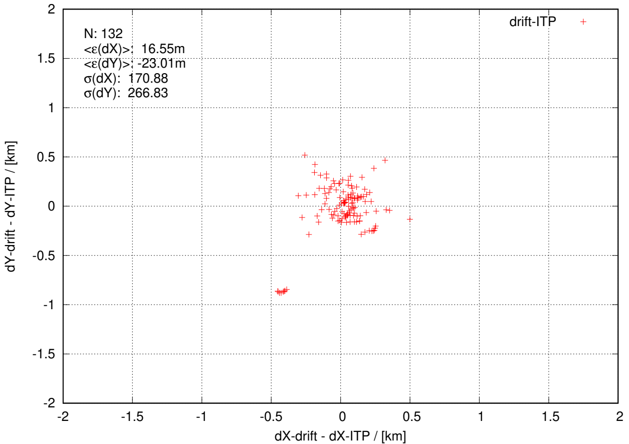
itp122 20230103 to 20230330
