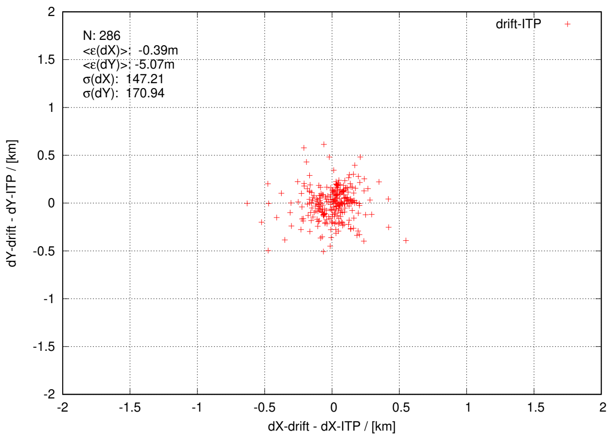
itp137 20230103 to 20230331
