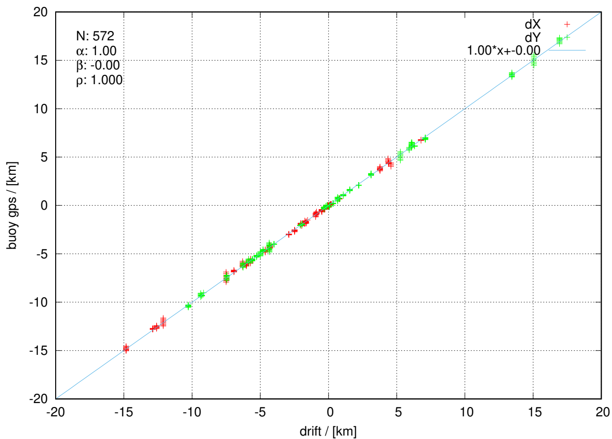
itp137 20230103 to 20230331
