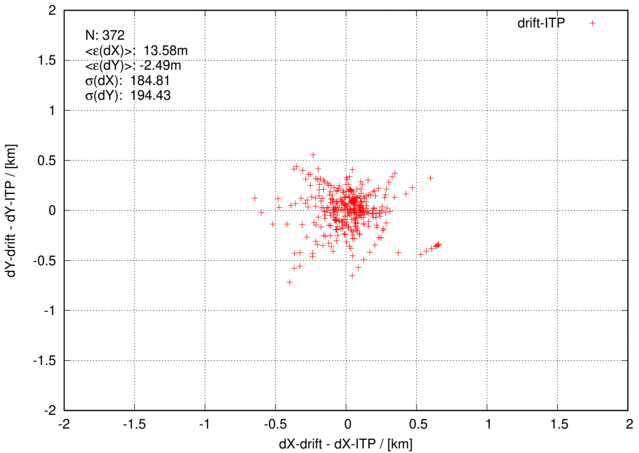
itp126 20230104 to 20230331
