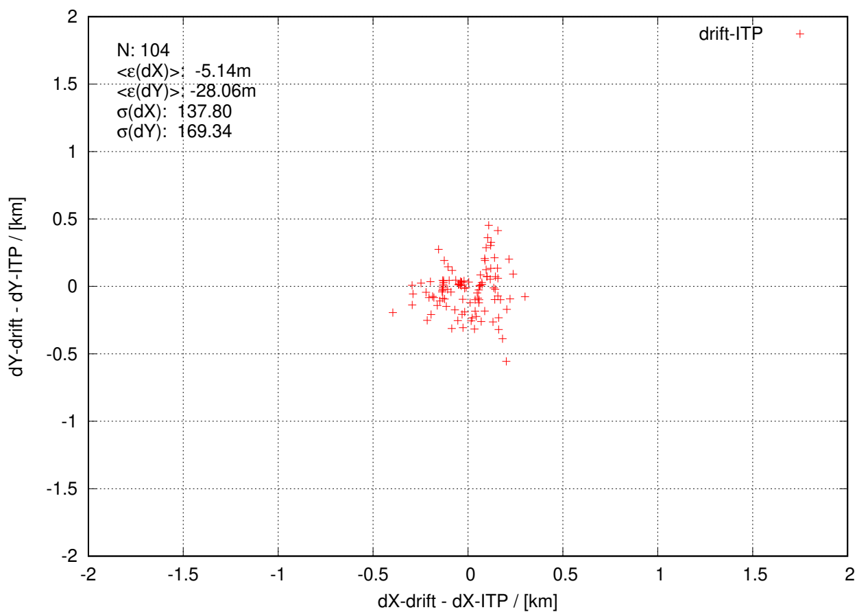
itp130 20230103 to 20230330
