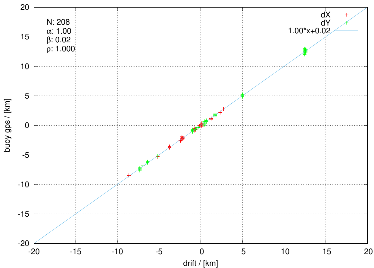
itp130 20230103 to 20230330
