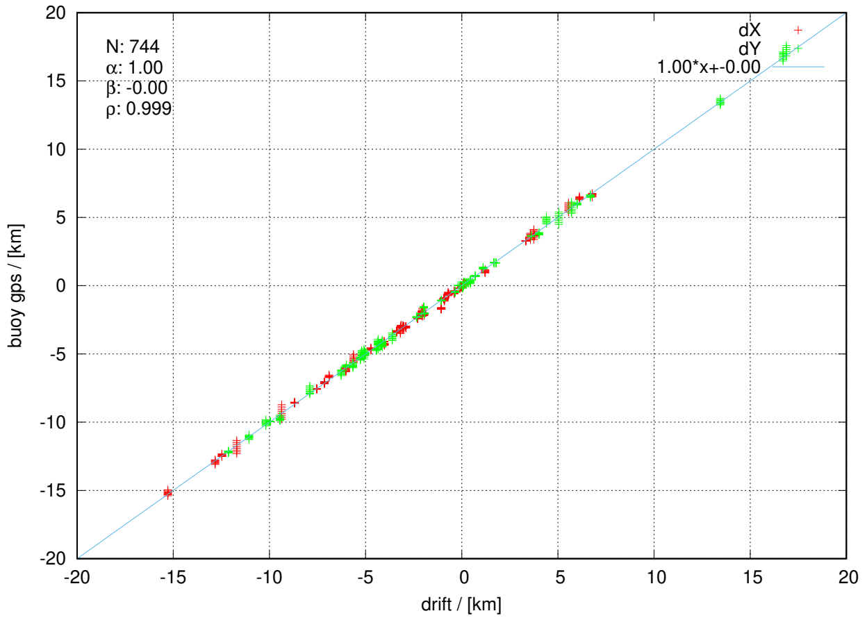
itp126 20230104 to 20230331
