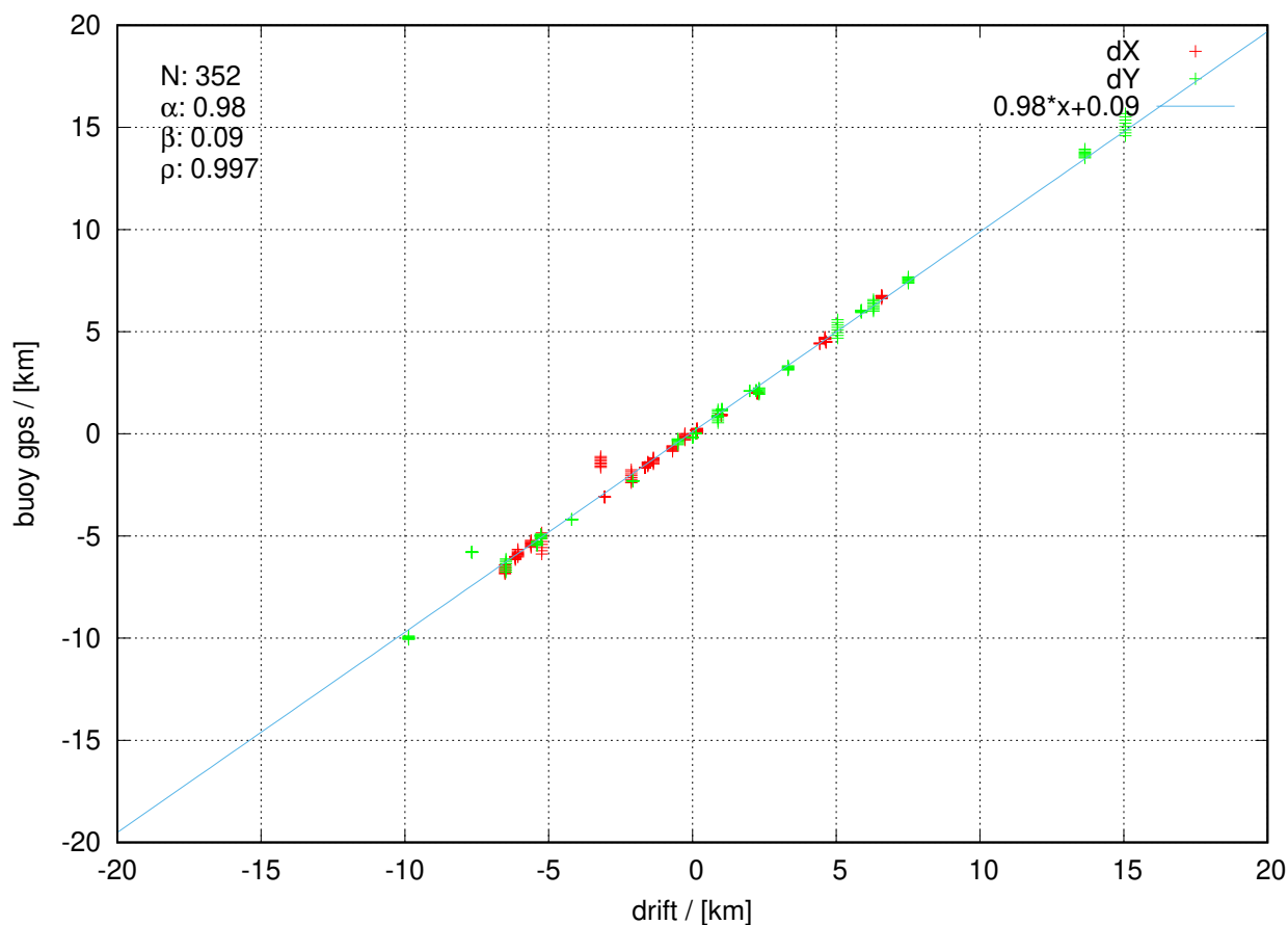
itp136 20230103 to 20230331
