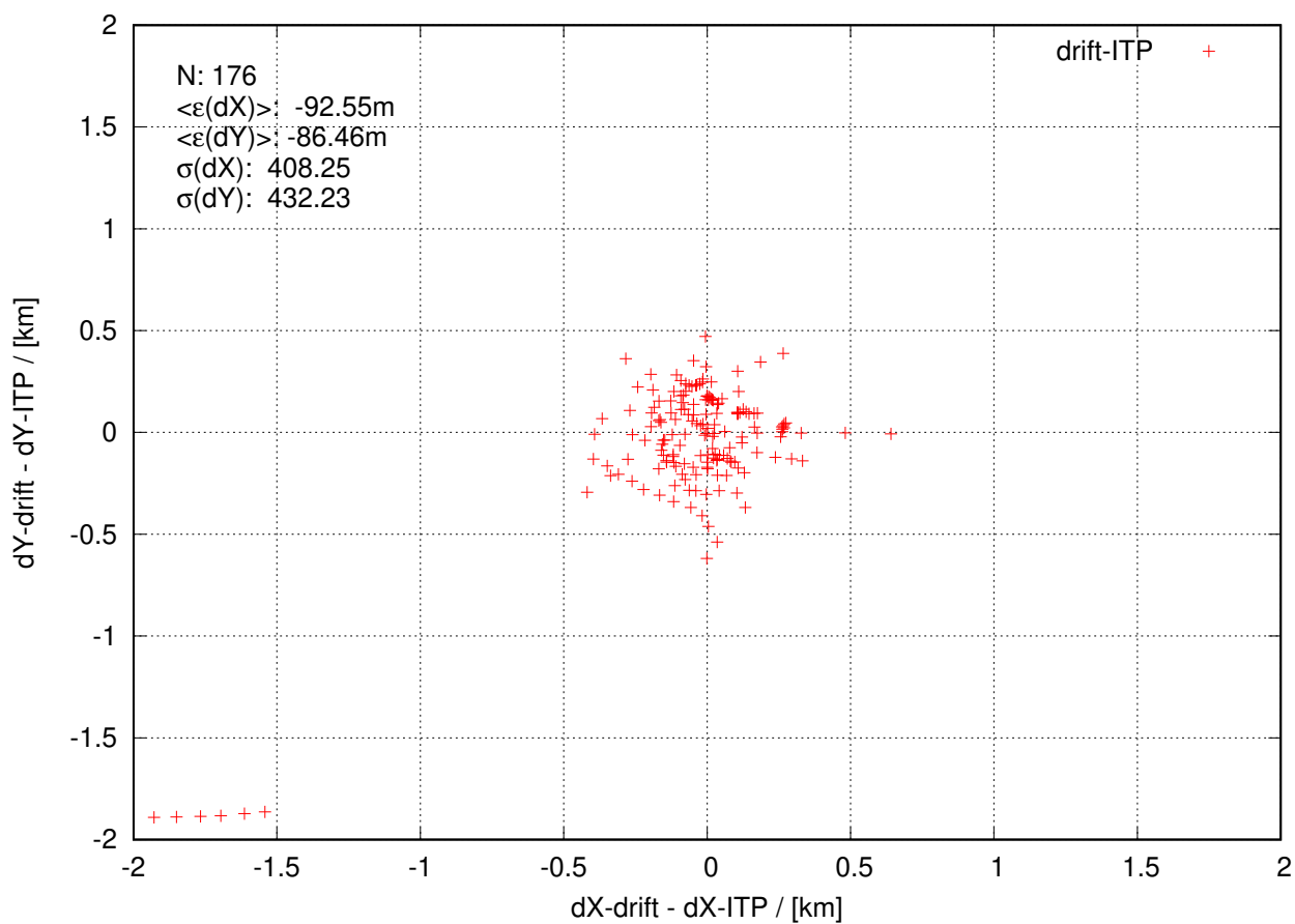
itp136 20230103 to 20230331
