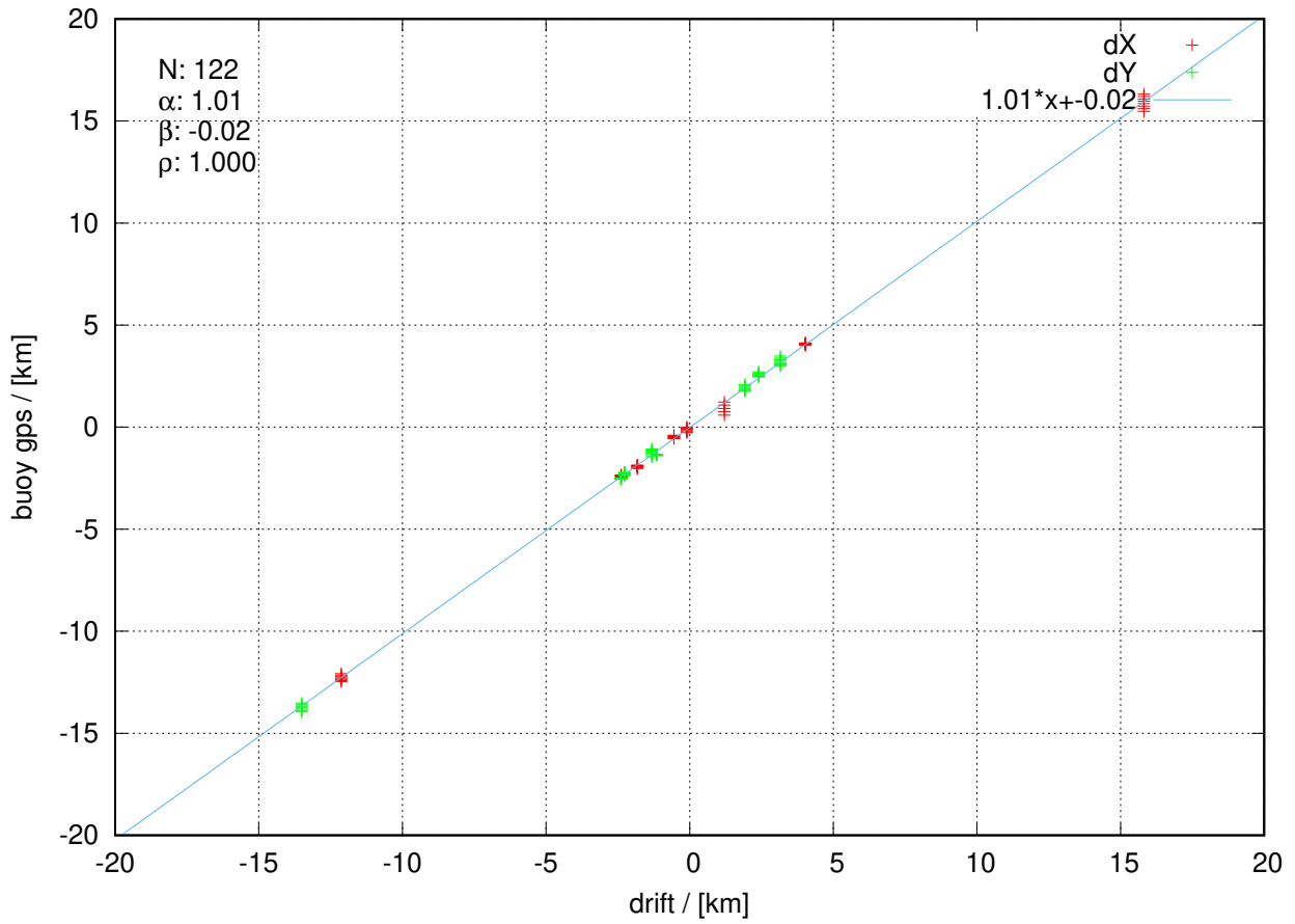
itp115 20230123 to 20230313
