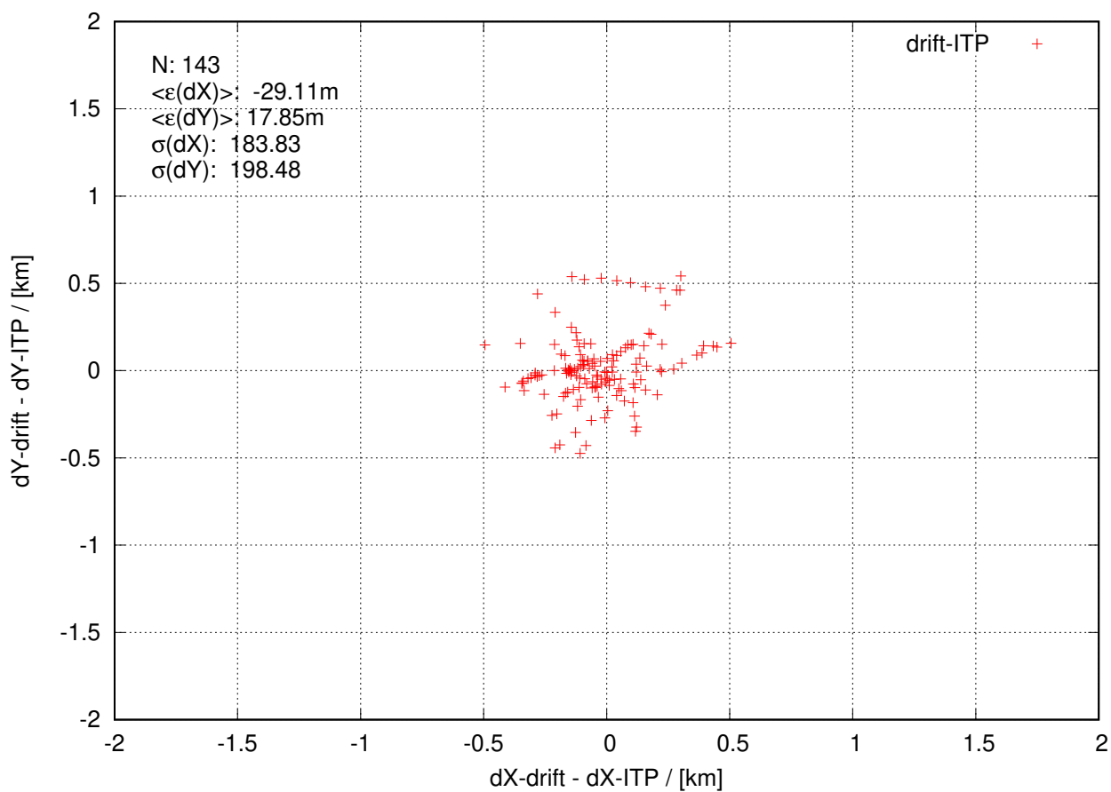
itp131 20230110 to 20230325
