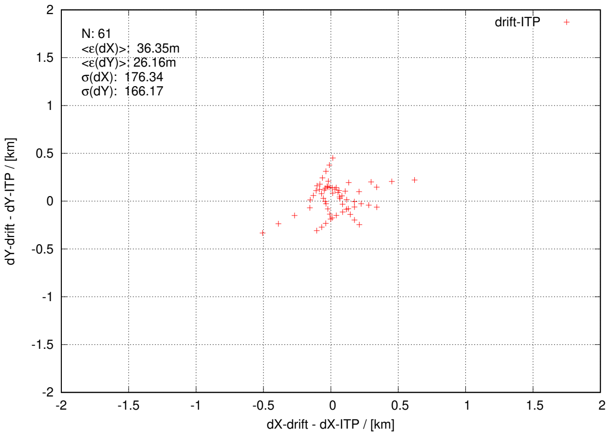
itp115 20230123 to 20230313
