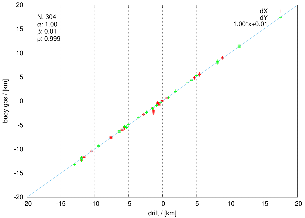
itp121 20230102 to 20230328
