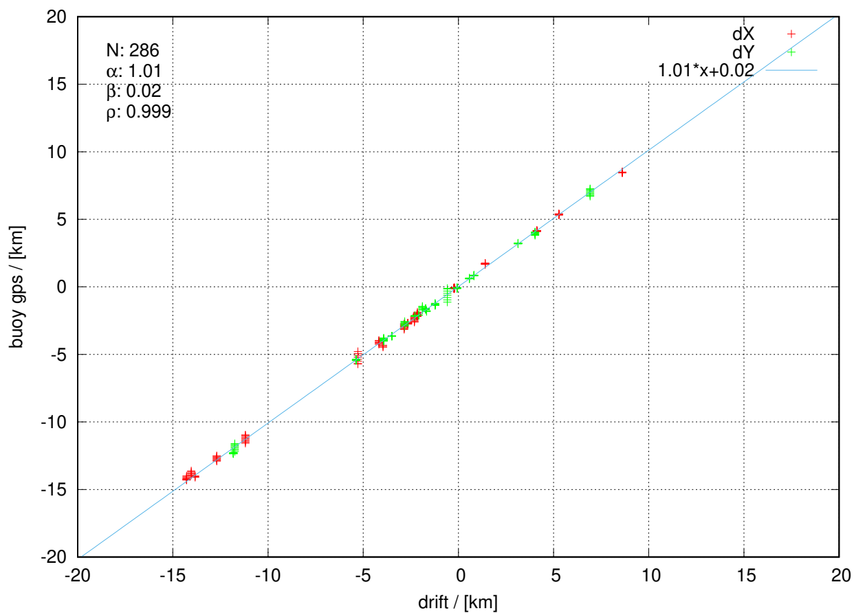
itp131 20230110 to 20230325
