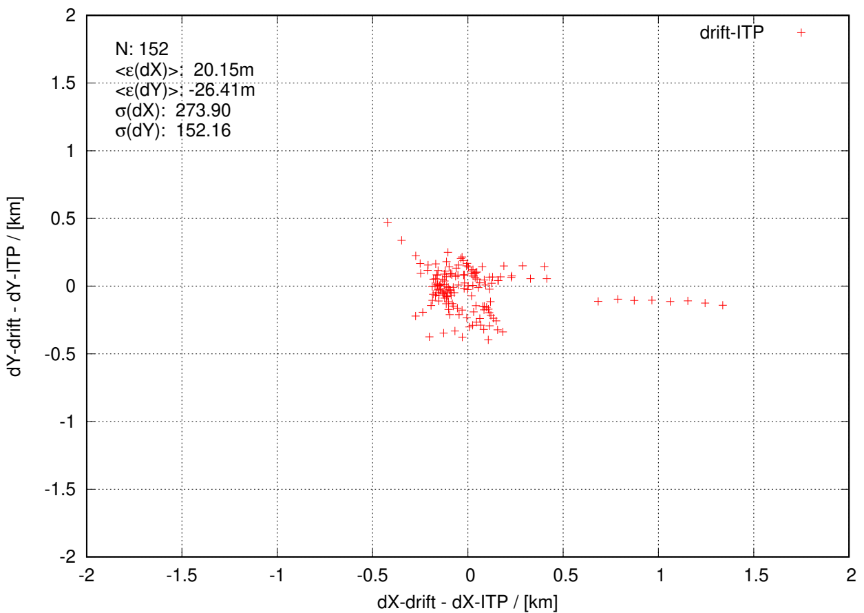
itp121 20230102 to 20230328
