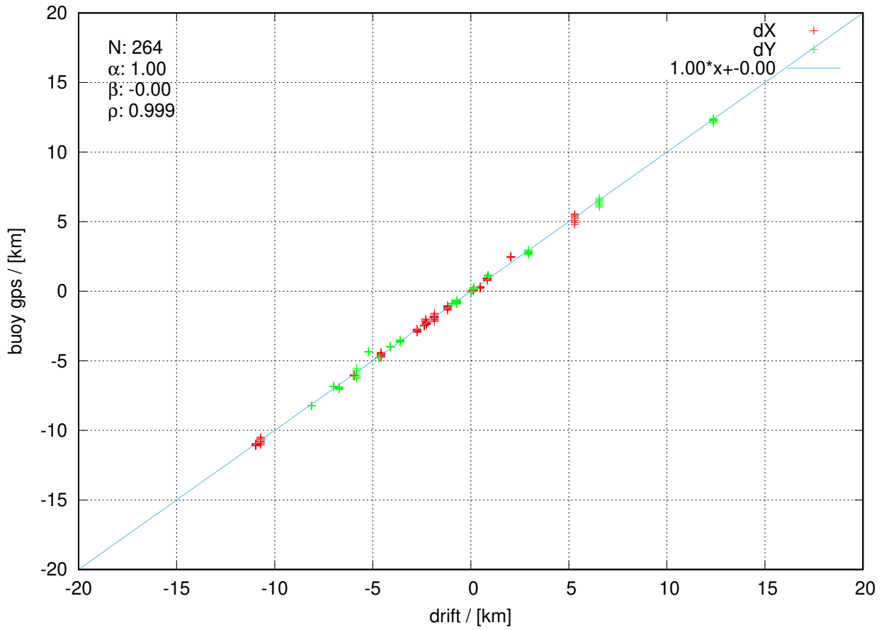
itp122 20230103 to 20230330
