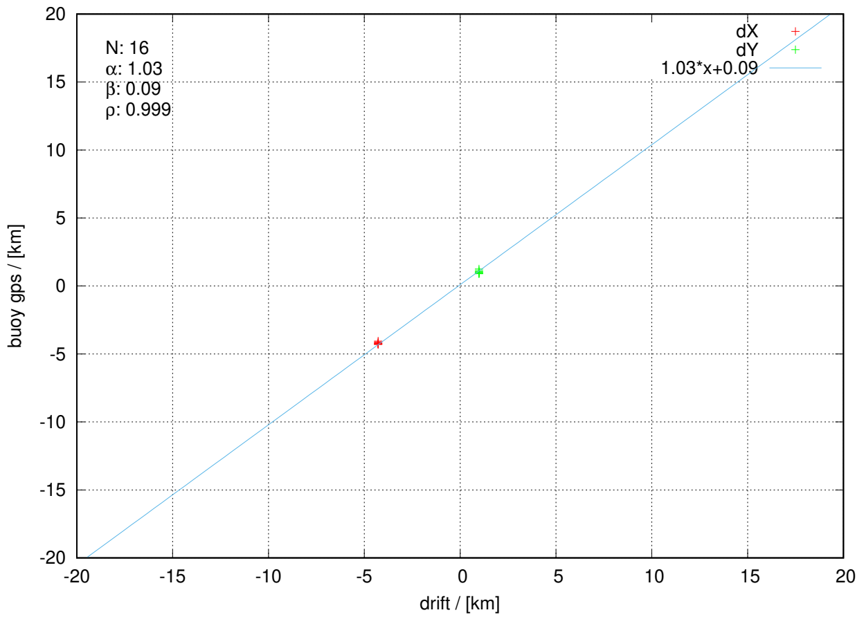
itp141 20231228 to 20231229
