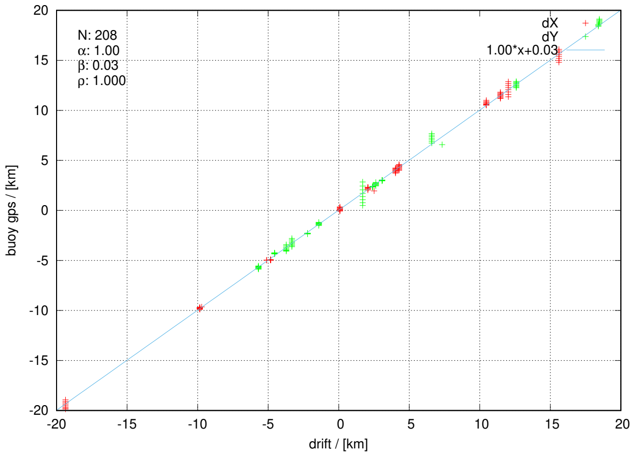
itp139 20231014 to 20231202
