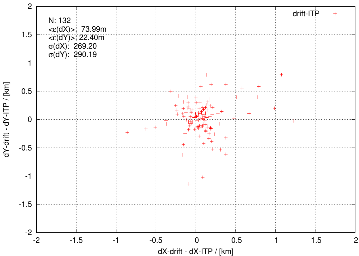
itp137 20230930 to 20231129
