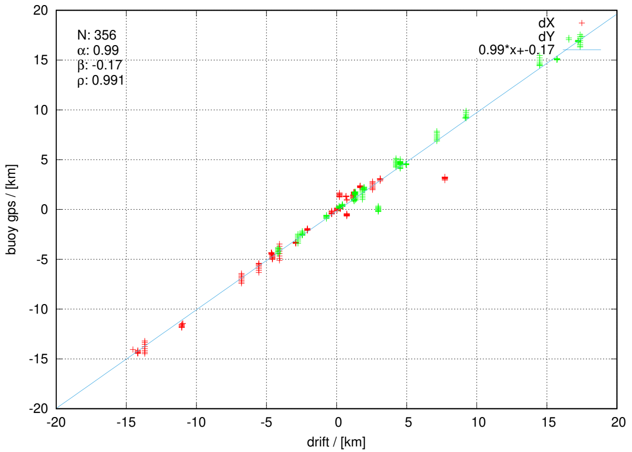
itp125 20230930 to 20231130
