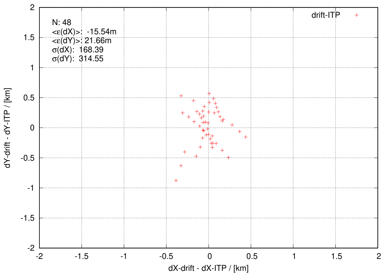
itp138 20231014 to 20231202
