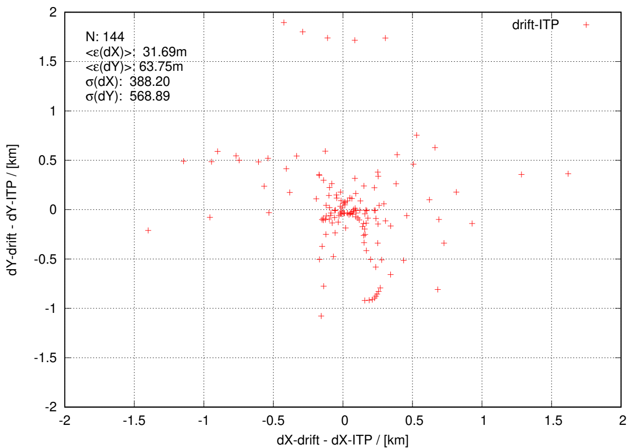
itp126 20230930 to 20231226
