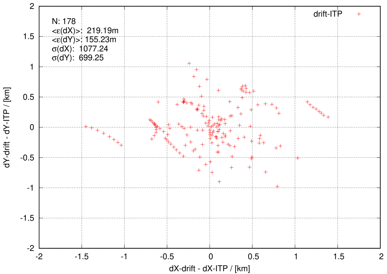
itp125 20230930 to 20231130
