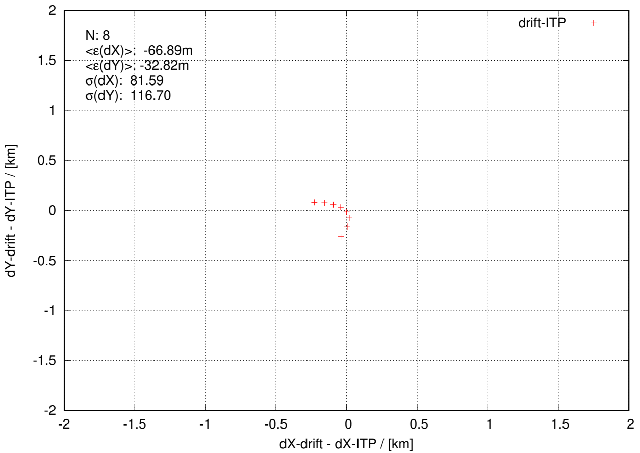
itp141 20231228 to 20231229
