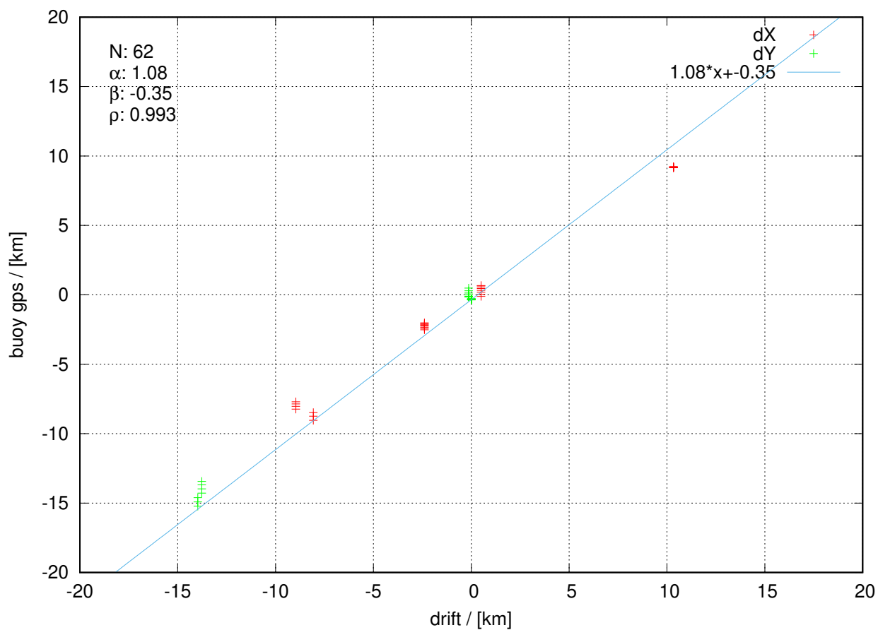
itp136 20231006 to 20231127
