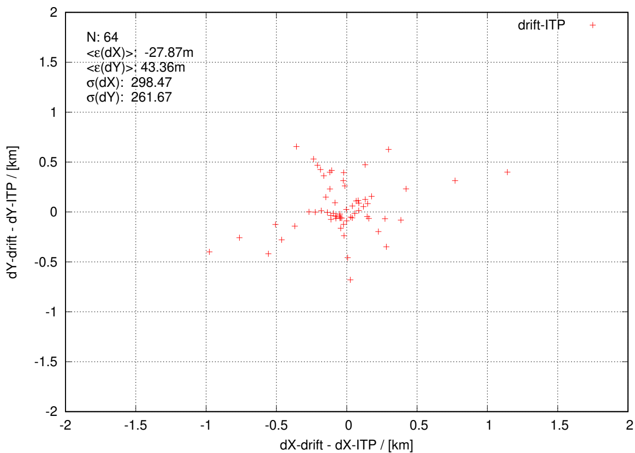
itp113 20231112 to 20231129
