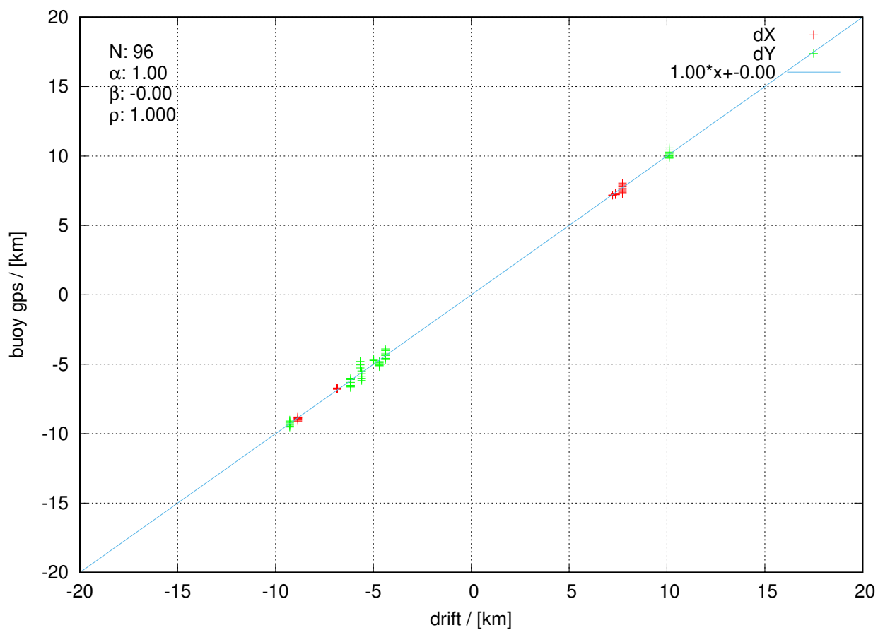
itp138 20231014 to 20231202
