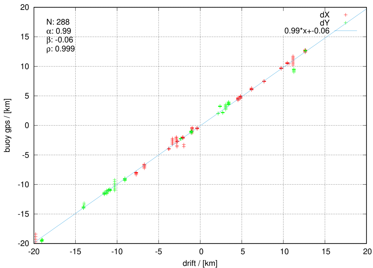
itp126 20230930 to 20231226
