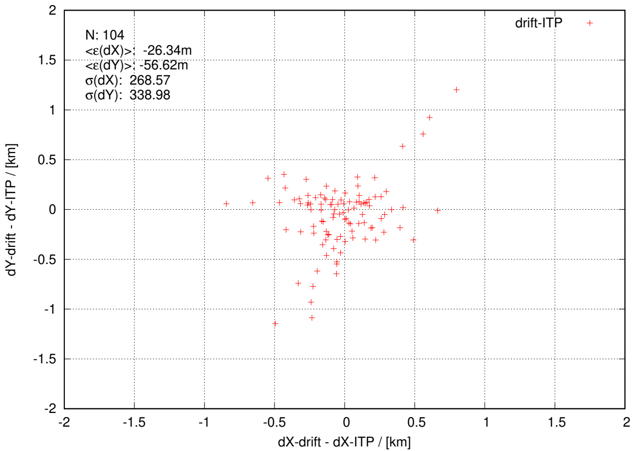
itp139 20231014 to 20231202
