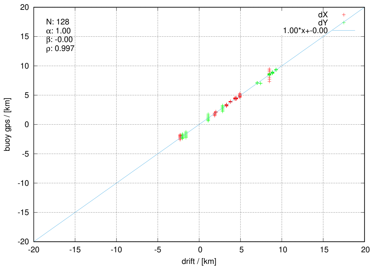
itp113 20231112 to 20231129
