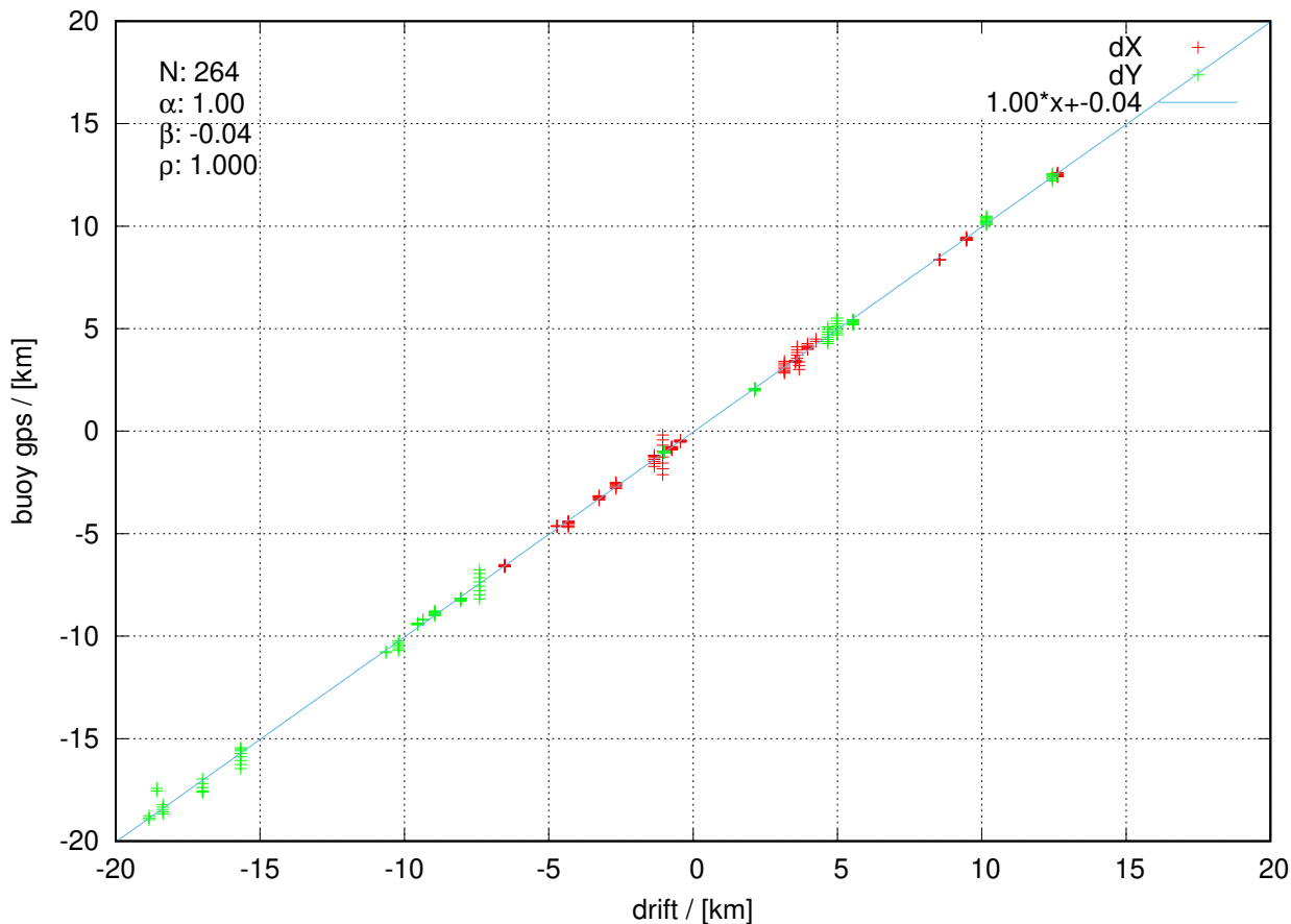
itp137 20230930 to 20231129
